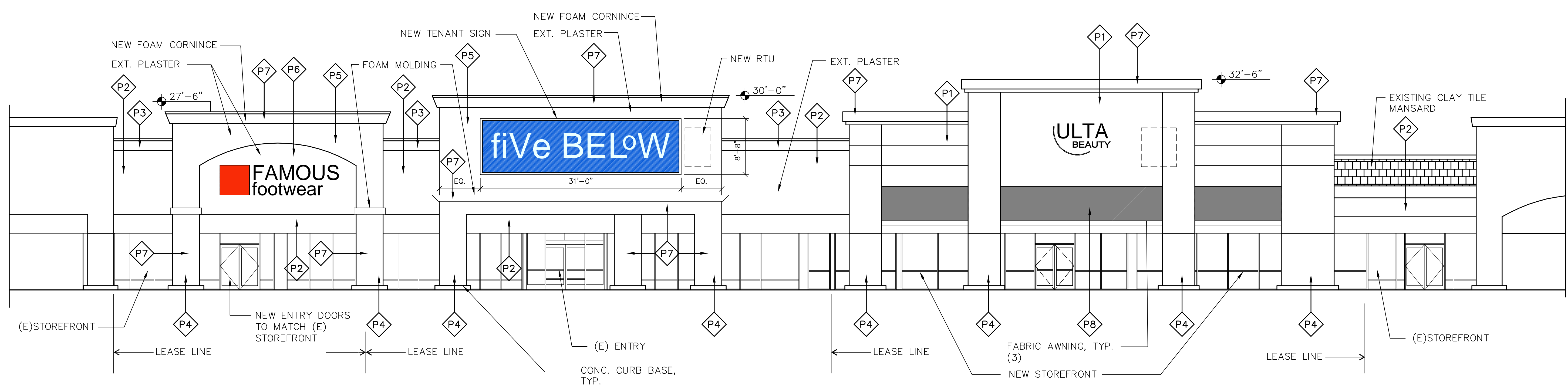
1 PROPOSED FRONT ELEVATION 1/8" = 1'-0"
