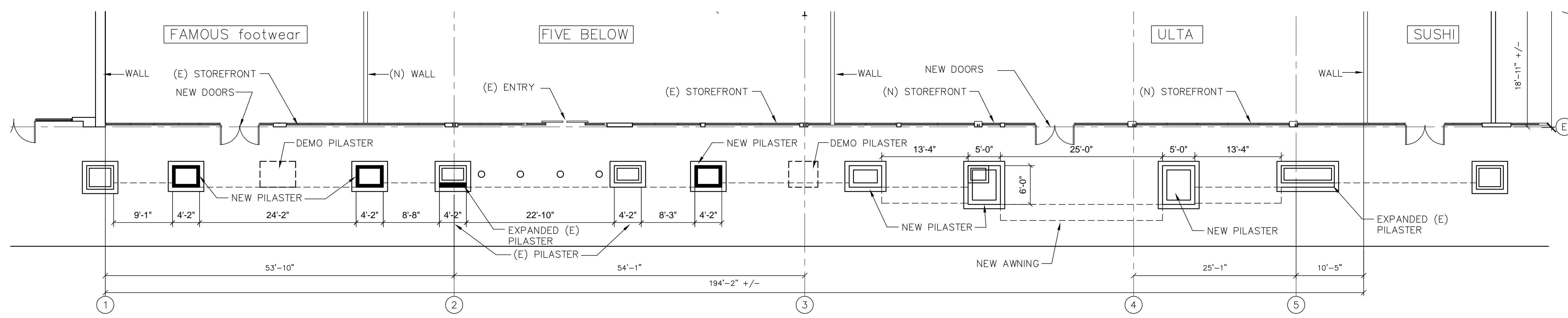
1 PROPOSED FRONT ELEVATION 1/8" = 1'-0"
