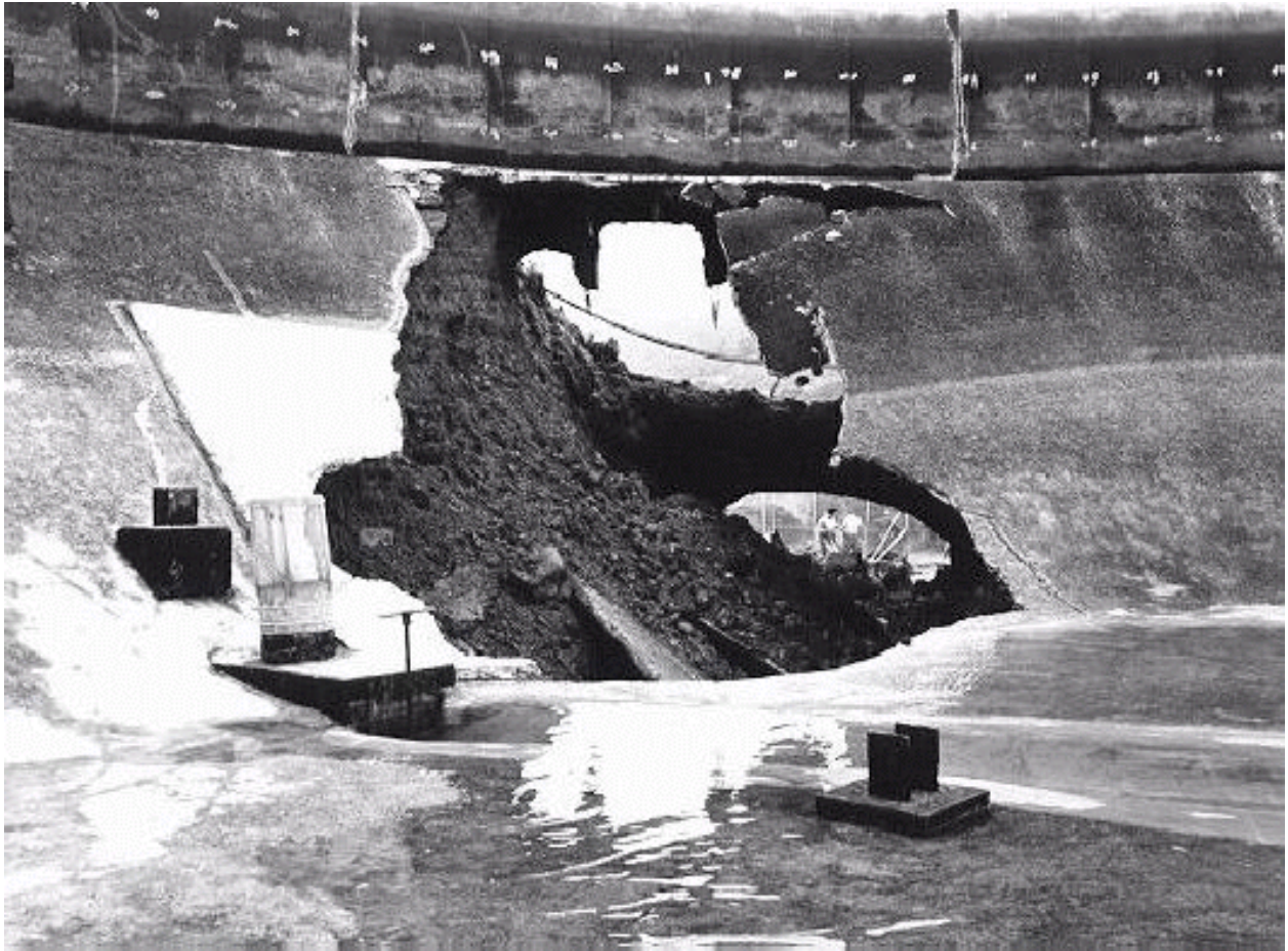
Lompoc Miguelito Canyon reservoir in 1969, which collapsed at one end and a million gallons of water gushed out. It was in the process of being refilled after repairs only one week earlier
